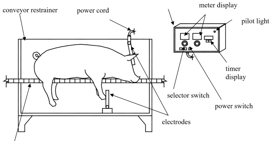
Figure 4 — Automatic stunner
