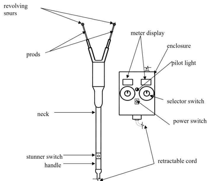
Figure 1 — Tong type head-only stunner
